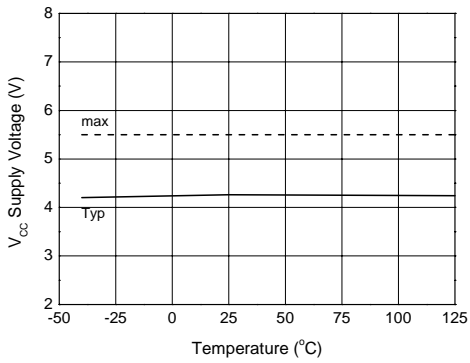
Figure 24a. VCC UnderVoltage Threshold (+) vs Temperature
