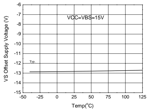
Figure 35. Maximum VS Negative Offset of vs Temperature
